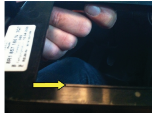
In AUDI Q5 cars, it will be necessary to file the inner plastic edge (back side of display cover) leaning on NAViPAD screen.
